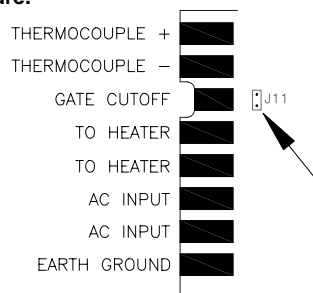
Figure 16 - Gate Cutoff Jumper, J11
