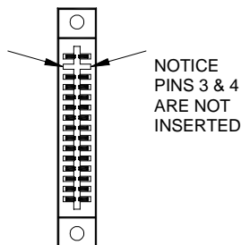
Figure 15 - Connector In Mainframe
