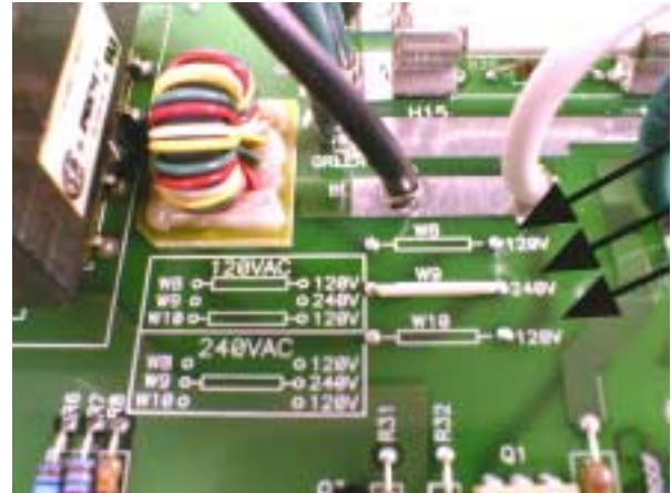
Figure 7 - Voltage Jumper Settings
