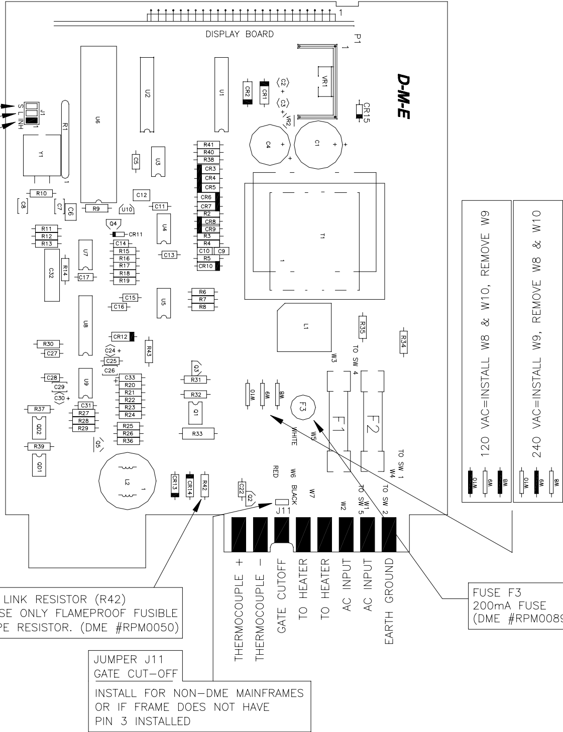
Figure 18 - Main Board Component Layout
