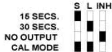
Figure 8 – 100% Power Jumper (J1) Settings
